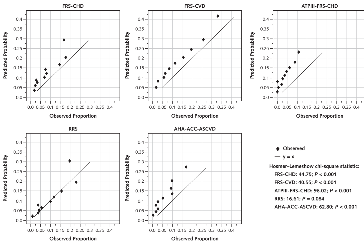
Figure 1. Risk score-specific predicted and observed events in men, by decile of calculated risk.
