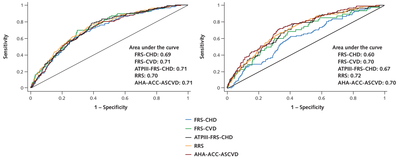
Appendix Figure. Area under the curve for all 5 risk prediction models.
