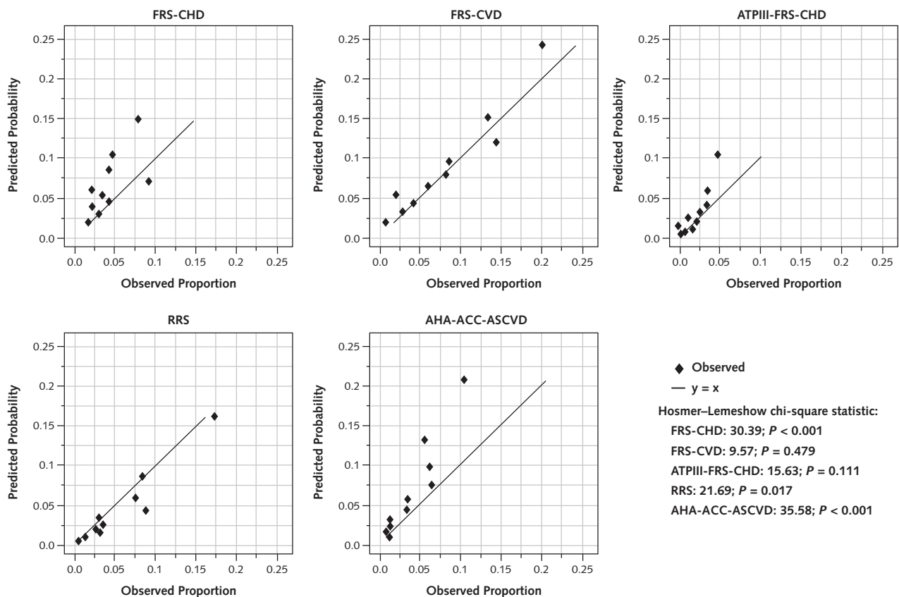
Figure 2. Risk score-specific predicted and observed events in women, by decile of calculated risk.
